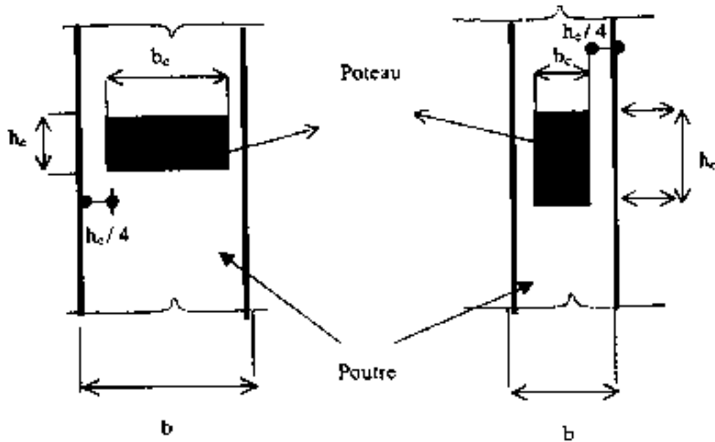
Figure 7.2 : Position poteau-poutre
