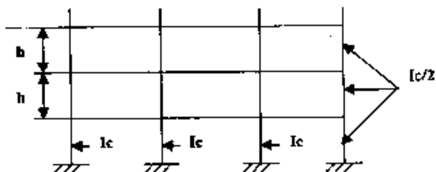
Figure 6.2 : Poutres - Poteaux
